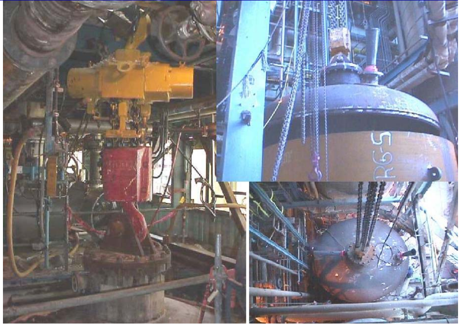
Rigging a paper mill digester vessel
