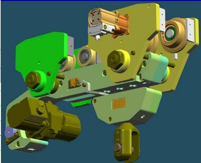
CAD Model of the new JDN Low Headroom Trolley LMF25T
